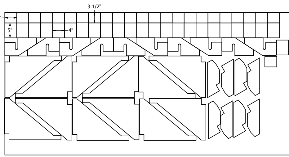
Cut 2 3/4" plywood
