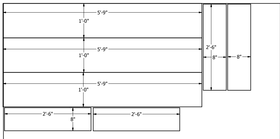
Cut 2 1/2" plywood
