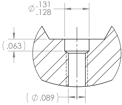
DETAIL D SCALE 4 : 1
