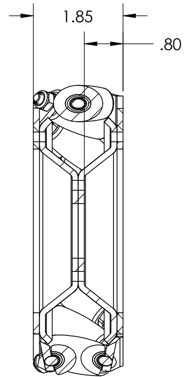
SECTION B-B
